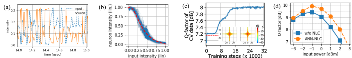
Fig. 2: (a) Waveforms of a training pattern and the corresponding neuron output captured by a real-time oscilloscope; (b) A snapshot of the activation function of a photonic neuron modulator at f_{\text{neuron}} = 194.776 THz with Lorentzian fitting (dotted line) (c) ANN-NLC training convergence with a Lorentzian activation function (inset: density plot of the input layer weights of the ANN-NLC model with 821 triplets); (d) Transmission performance for an execution frame of a 32 Gbaud PM-16QAM signal over a 10,080 km PSCF transmission link.
