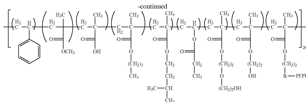
P[(S-MMA-MAA-BMA-iPMA-VP-HEGEMA-HEMA)-g-PFPE] 26
