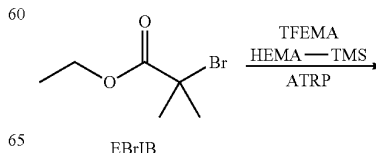
Scheme 3. Synthetic route for P(TFEMA-co-HEMA)-g-PFPE
