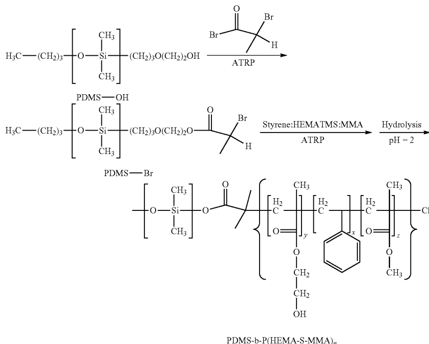
Scheme 6. Synthetic pathway toward PDMS-b-(HEMA-S-MMA) n .
