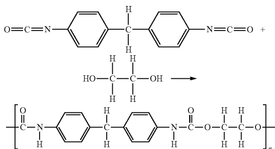
Scheme 1. Synthesis of a traditional linear polyurethane (PU)
