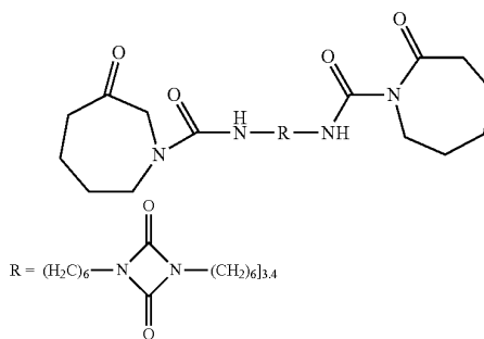
The Chemical Structure of Desmodur BL 3272, a Polyisocyanate that has \epsilon -Caprolactam Protecting Groups
